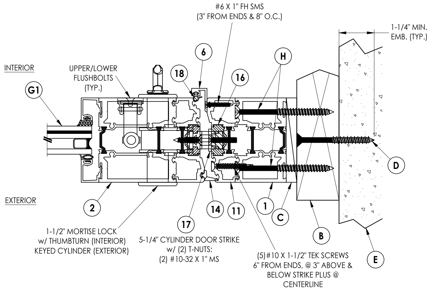
2 5 HORIZONTAL CROSS SECTION Shown w/ 2X Buck
