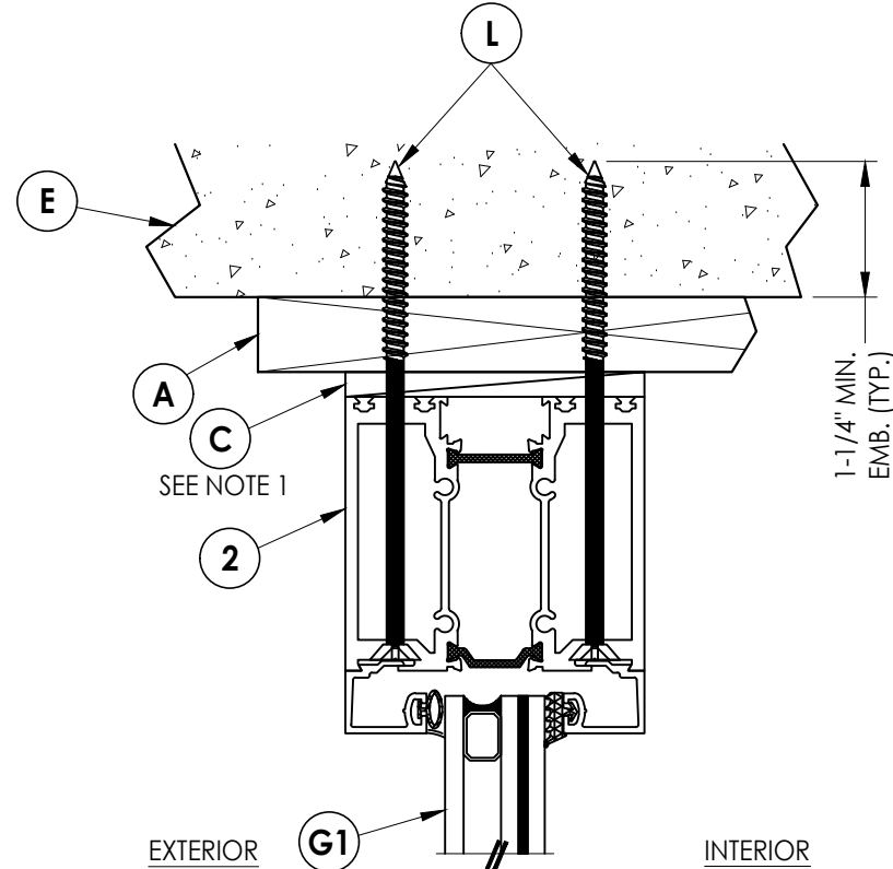
2 6 VERTICAL CROSS SECTION Shown w/ 1X Buck
