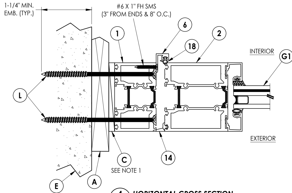
4 6 HORIZONTAL CROSS SECTION Shown w/ 1X Buck
