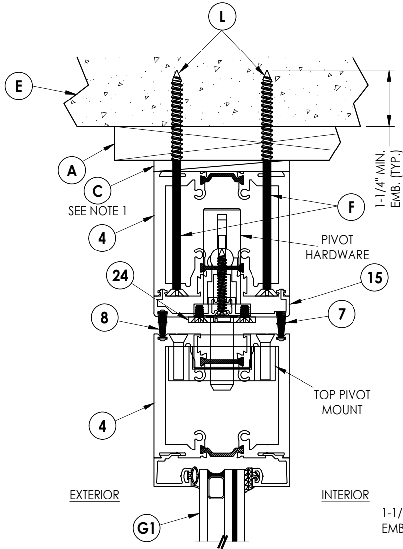
1 6 VERTICAL CROSS SECTION Shown w/ 1X Buck
